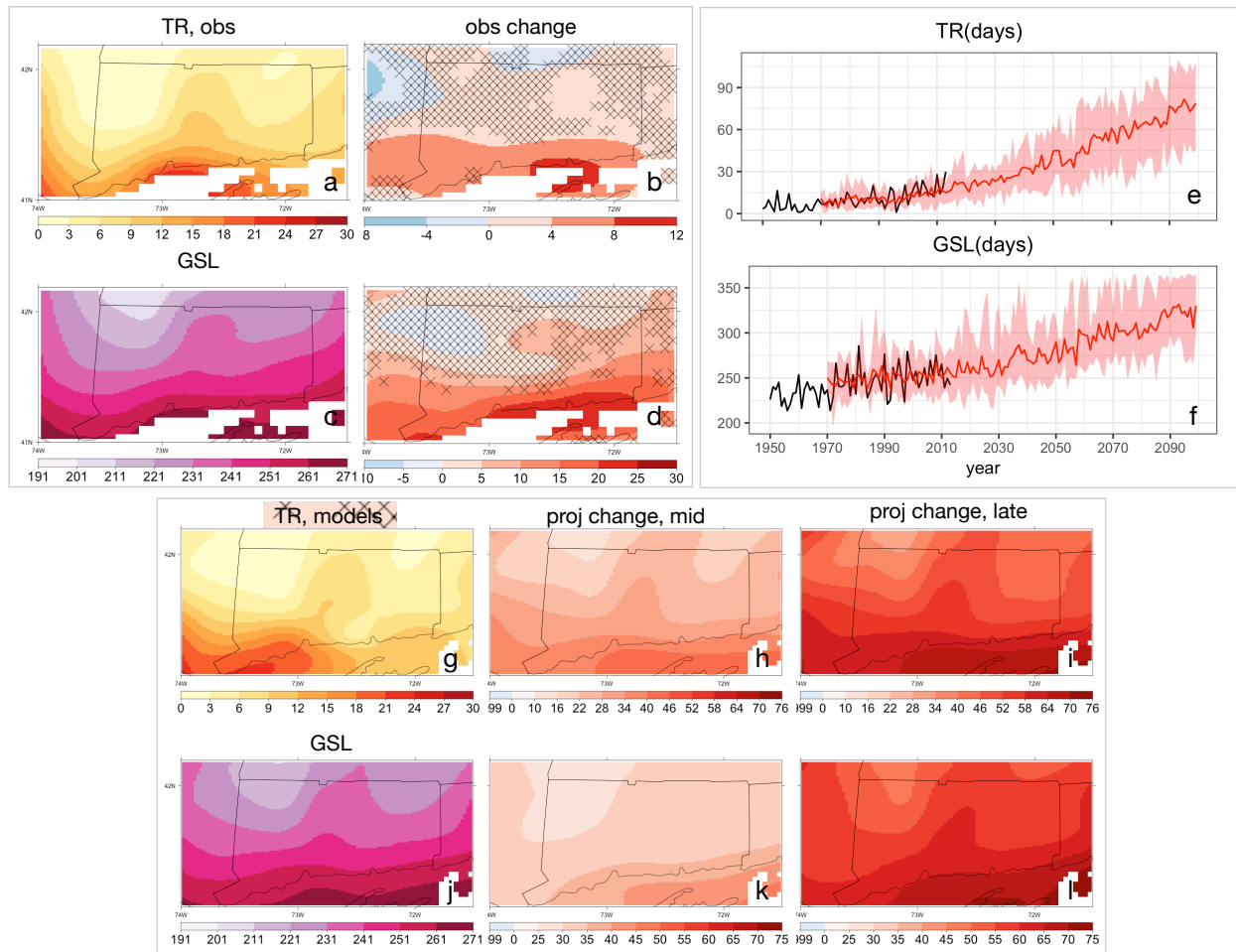
Figure A-3.4 (a-d) Observed changes in nighttime warm weather indices, TR, GSL; (e,f) Time series of nighttime warm weather indices; (g-l) Projected changes nighttime warm weather indices.
