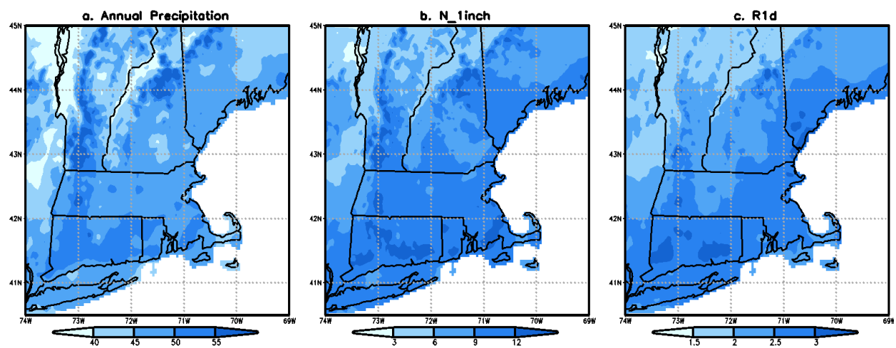
Figure A-4.1 Observed annual precipitation (inches), N_1inch (days), and R1d (inches) for the reference period (1970-1999).
