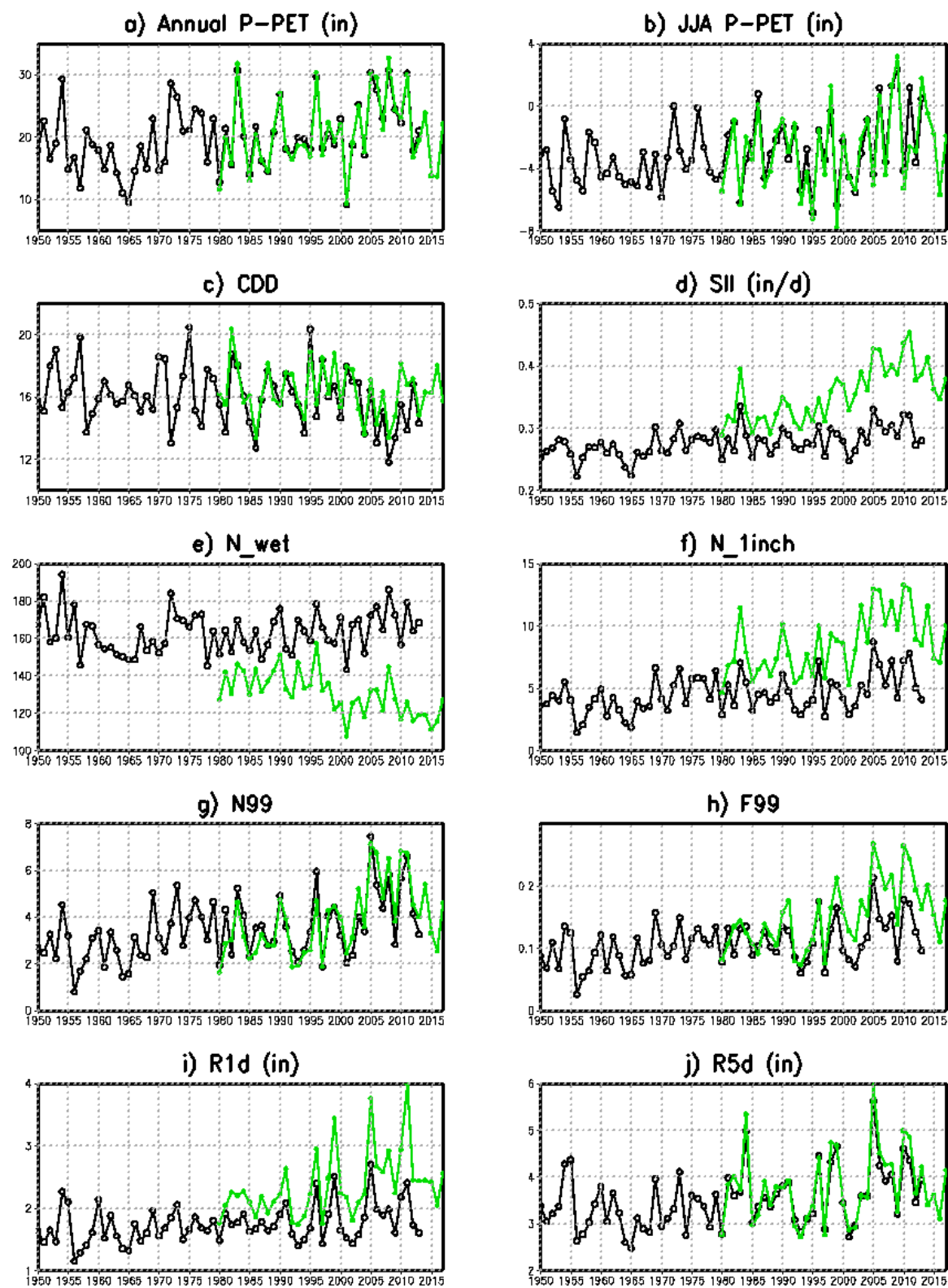
Figure A-4.2 Observed time series of precipitation indices comparison from the two datasets, averaged over the Northeast region.
