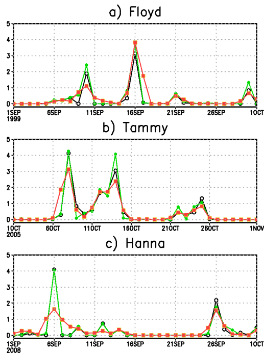
Figure A-2.1 Time series of daily precipitation (inches) during three extreme events associated with Hurricanes (a) Floyd, (b) Tammy, and (c) Hanna from two datasets of gridded daily observations: METDATA (green) and Livneh (red), and from meteorological stations (black).
