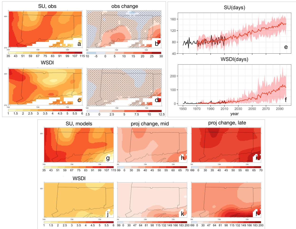
Figure A-3.3 (a-d) Observed changes in Daytime warm weather indices (SU, WSDI); (e,f) Time series of Daytime warm weather indices; (g-l) Projected changes in Daytime warm weather indices.
