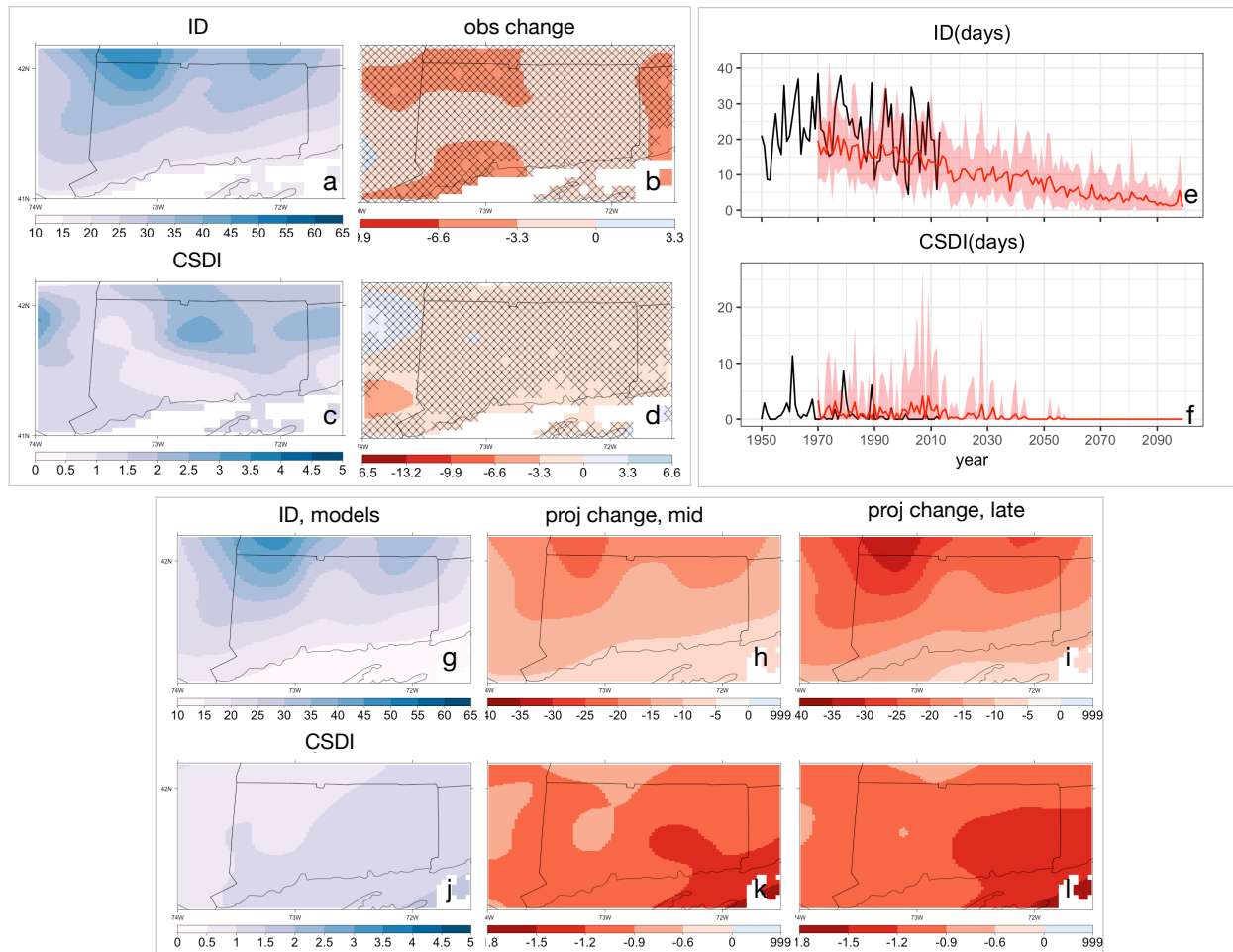
Figure A-3.5 (a-d) Observed changes in daytime cold weather indices (ID, CSDI); (e,f) Time series of daytime cold weather indices; (g-l) Projected changes in daytime cold weather indices.
