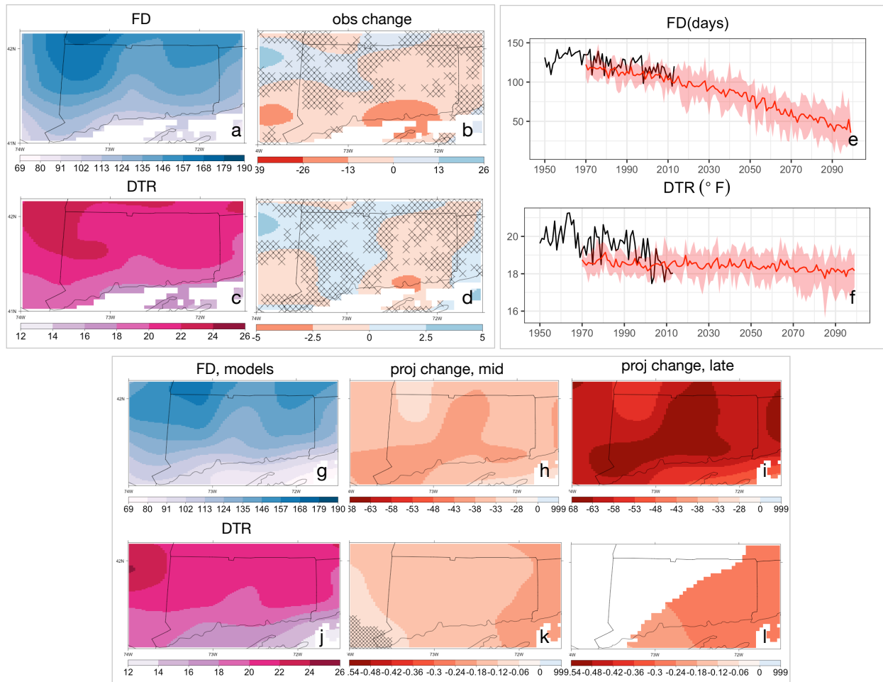
Figure A-3.6 (a-d) Observed changes in nighttime cold weather indices (FD, DTR); (e,f) Time series of nighttime cold weather indices; (g-l) Projected changes nighttime cold weather indices.
